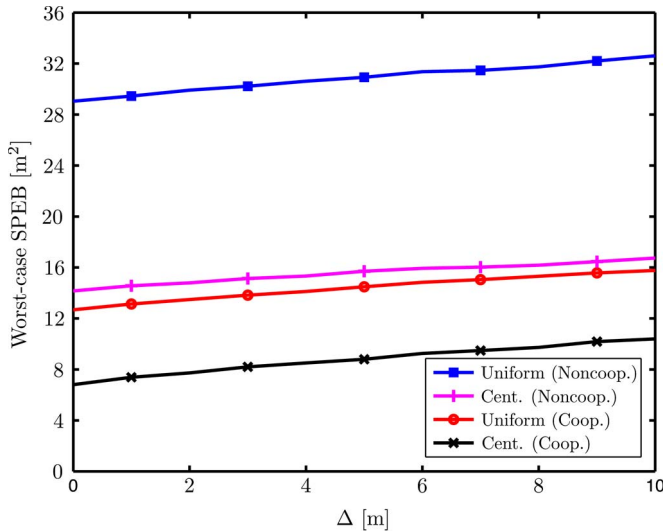
Fig. 8. Worst-case SPEB with respect to USS by the centralized strategy and the uniform strategy. In the cooperation setting, P_{\text{agt}}^{\text{tot}} = 1.25 W.
