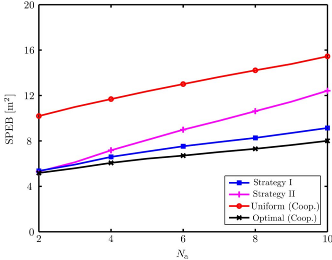
Fig. 7. Average SPEB with respect to the number of agents by different strategies for P_{\text{agt}}^{\text{tot}} = 2.5 W.
