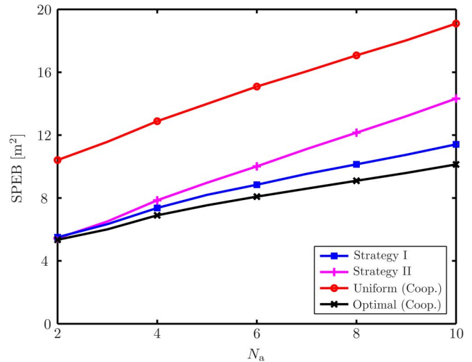
Fig. 6. Average SPEB with respect to the number of agents by different strategies for P_{\text{agt}}^{\text{tot}} = 1.25 W.
