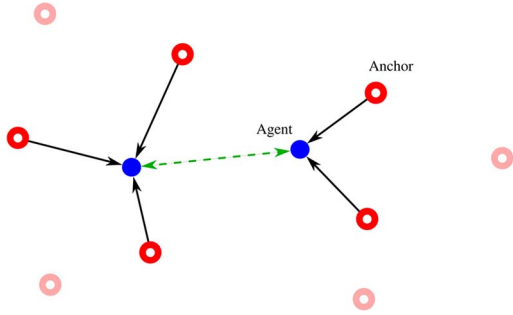
Fig. 3. Sparsity property of the optimal APAV: for each agent, the optimal localization accuracy can be achieved with at most three activated anchors.
