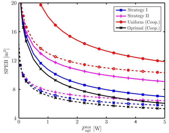
Fig. 5. Average SPEB with respect to P_{\text{agt}}^{\text{tot}} . Two cases for different N_a are considered: N_a = 4 (dashed lines) and N_a = 8 (solid lines).
