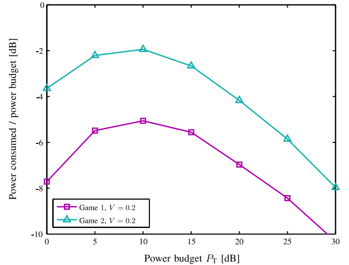
Fig. 6. Average power consumed over all the agents under the power budget P_T for P^{(k)} = P_T, \forall k .
