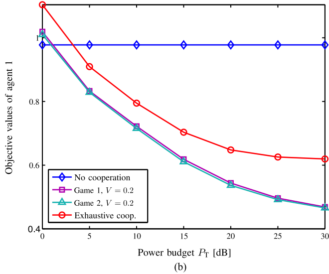
Fig. 7. MSE of the estimated position and the objective value of agent 1 versus the power budget P_T under P^{(k)} = P_T, \forall k .
