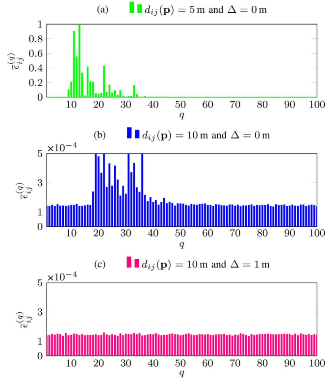
Fig. 4. Energy vectors for different values of signal path-length d_{ij}(\mathbf{p}) and total wall thickness \Delta . Energy values are normalized to the maximum of the vector in (a). Results are obtained with an ED setting and channel model used in the case study (see Section VI).
